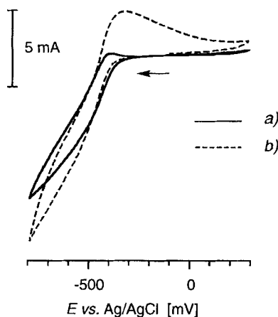
Fig. 9. Cyclic voltammograms of flavo-thiazolio-cyclophane 6 (5 mM) in a 50 mM soln. of \text{Et}_4\text{NBr} in \text{MeOH}/\text{Et}_3\text{N} 50:1 (v/v) at a) a glassy carbon counter electrode and b) a Pt wire counter electrode. Scan rate: 20 \text{ mV s}^{-1} , 308 K, Pt foil ( 50 \times 12 \times 10 \text{ mm} ) working electrode.
