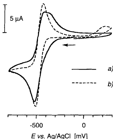
Fig. 5. Cyclic voltammograms of flavo-thiazolio-cyclophane 6 (1 mM) in a 50 mM \text{Et}_4\text{NBr} soln. a) in MeOH and b) in MeOH/ \text{Et}_3\text{N} 100:1 (v/v), recorded 1 h after addition of \text{Et}_3\text{N} . Scan rate 20 \text{ mV s}^{-1} , 300 K, glassy carbon working electrode.
