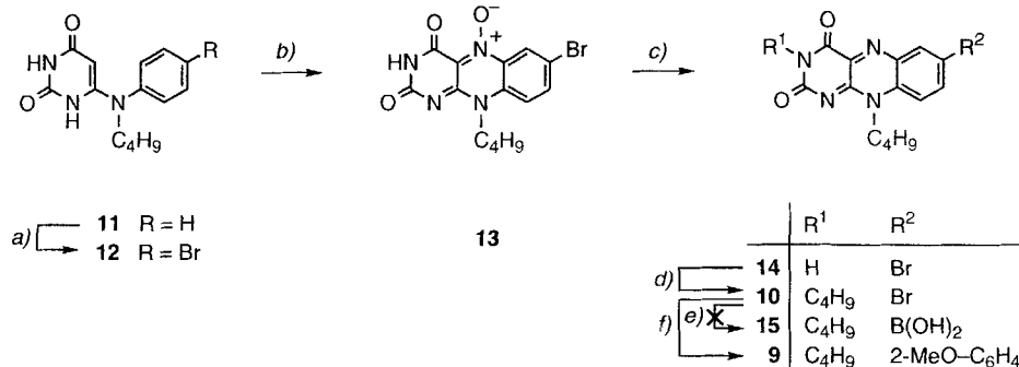
Scheme 2. Synthesis of 7-Arylflavin 9
