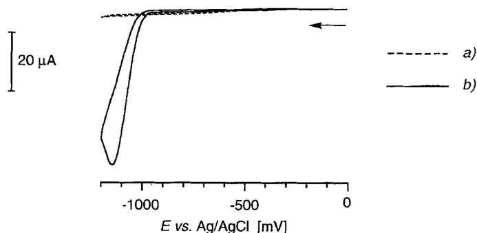
Fig. 10. Cyclic voltammograms of a) benzaldehyde (1 mM) and b) 4-formylbenzonitrile (1 mM) in a 50 mM soln. of \text{Et}_4\text{NBr} in \text{MeOH}/\text{Et}_3\text{N} 100:1 (v/v). Scan rate 20 \text{ mV s}^{-1} , 308 K, glassy carbon working electrode.
