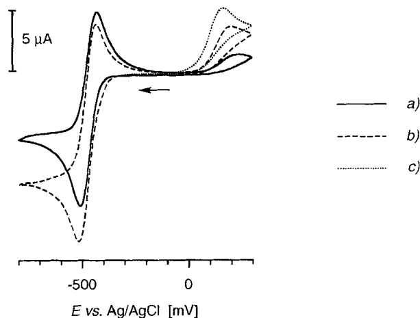
Fig. 6. Cyclic voltammograms of a) flavo-thiazolio-cyclophane 6 (1 mM), b) flavo-thiazolio-cleft 7 (1 mM), and c) 3-benzyl-4-methylthiazolium bromide 8 (1 mM) in a 50 mM soln. of \text{Et}_4\text{NBr} in \text{MeOH}/\text{Et}_3\text{N} 100:1 (v/v). Scan rate 20 \text{ mV s}^{-1} , 300 K, glassy carbon working electrode.
