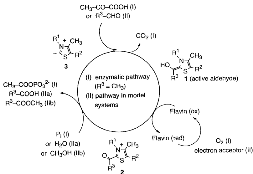
Scheme 1. Catalytic Cycles for the Conversion of Pyruvate to Acetyl Phosphate Catalyzed by Pyruvate Oxidase (Pathway I) and for the Oxidation of an Aldehyde to a Carboxylic Acid (Pathway IIa) or Methyl Ester (Pathway IIb) in Model Systems
