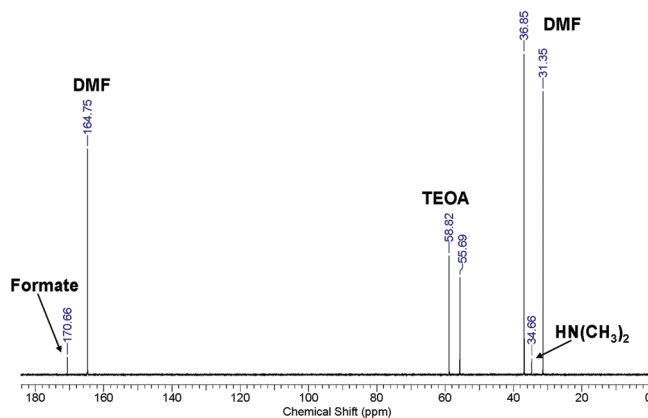
Figure 3. ^{13}\text{C} NMR ( \text{D}_2\text{O} , 600 MHz) of a 5:1 DMF/TEOA mixture containing 75 vol % \text{H}_2\text{O} .
