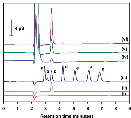
Figure 1. Increase in the formate levels with the water concentration for 5:1 DMF/TEOA solutions stored for 2 h: (i) blank, \text{H}_2\text{O} ; (ii) 10^{-4} M formate; (iii) standard 10^{-4} M anion mixture; (iv) DMF/TEOA + 30 vol % \text{H}_2\text{O} ; (v) DMF/TEOA + 50 vol % \text{H}_2\text{O} ; (vi) DMF/TEOA + 75 vol % \text{H}_2\text{O} . Chromatographic conditions as described in the Supporting Information. Peak assignment: (a) fluoride; (b) acetate; (c) formate; (d) chloride; (e) nitrite; (f) nitrate; (g) bromide. The void is the result of a change in the absorbance related to the detection of unretained components of the injection.
