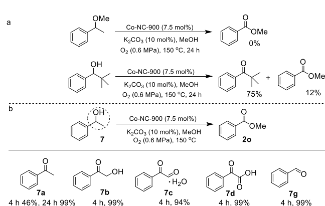
Scheme 7. Control experiments. a) The role of different functional groups in secondary alcohols was clarified. b) Reactions of 1-phenylethanol derivatives.
