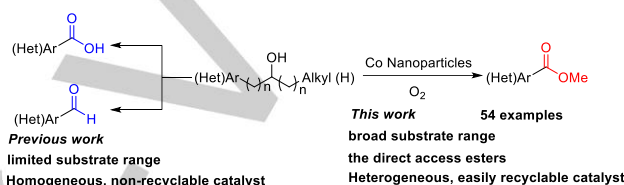
Scheme 1. Successive C-C bond cleavage of alcohols.
