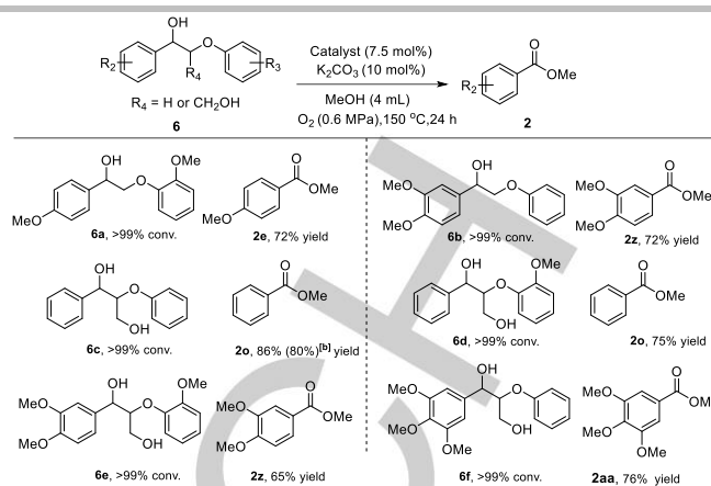
Scheme 6. Substrate Scope of lignin model compounds. Reaction conditions: lignin model compounds (0.25 mmol), K 2 CO 3 (10 mol%), Co-NC-900 (7.5 mol%), MeOH (4 mL), 0.6 MPa O 2 , 150 °C, 24 h. [b] Isolated yield.
