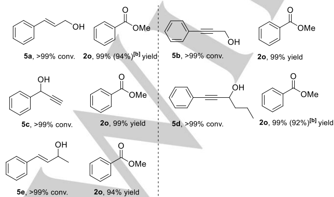
Scheme 5. Substrate Scope of allylic and propargylic alcohols. Reaction conditions: alcohol (0.25 mmol), K 2 CO 3 (10 mol%), Co-NC-900 (15 mol%), MeOH (4 mL), 0.6 MPa O 2 , 150 °C, 48 h. [b] Isolated yield.
