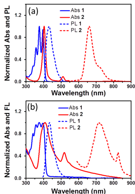
Figure 3. (a) Normalized absorption and emission spectra of \text{CHCl}_3 solution of 1 ( \lambda_{\text{ex}} = 375 nm, 0.1 mM) and 2 in deaerated \text{CHCl}_3 ( \lambda_{\text{ex}} = 510 nm, 0.1 mM). (b) Normalized absorption and emission spectra of liquid 1 ( \lambda_{\text{ex}} = 375 nm) and cast film of 2 ( \lambda_{\text{ex}} = 520 nm).
