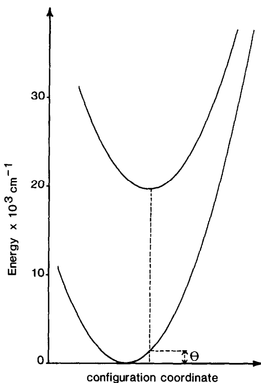
FIG. 7. Single-configurational-coordinate diagram for \text{Ba}_3\text{Ga}_2\text{S}_6:\text{Eu} ( x = 0.01 ). \hbar\omega = 300\text{ cm}^{-1} , and \theta = 1200\text{ cm}^{-1} (offset parameter: a_{uv} = 4 ).
