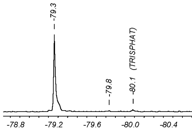
Fig. 4. ^{31}\text{P} -NMR spectrum (162 MHz, \text{DMSO}-d_6 ) of [\text{nBu}_3\text{NH}][\mathbf{5a}] .
