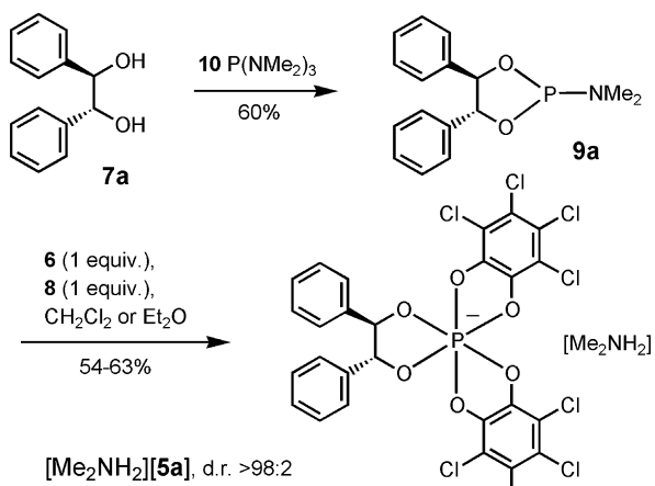
Fig. 7. Two-steps synthesis of [Me 2 NH 2 ][5a] via hydrobenzoin phosphoramidite 9a .
