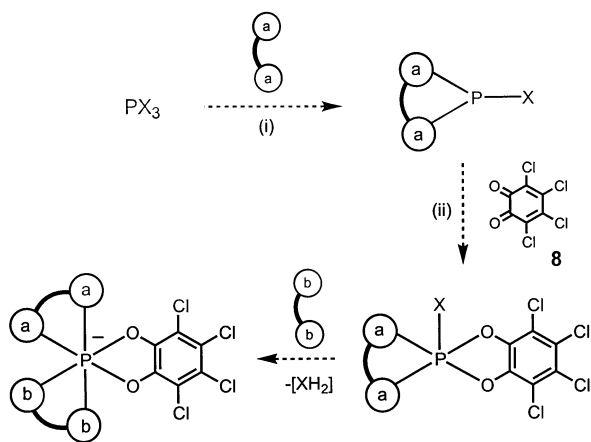
Fig. 6. Outline of the envisioned synthetic strategy for making of [XH 2 ][P(aa) 2 bb] salts.
