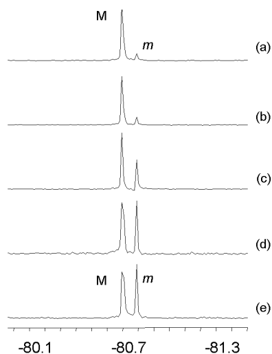
Fig. 8. Epimerization of [\text{Me}_2\text{NH}_2][\mathbf{5a}] as a function of time. ^{31}\text{P} -NMR (162 MHz, \text{MeOH}-d_4 ) (a) 1.5 h., d.r. 88:11; (b) 2.3 h.; d.r. 86:14; (c) 9.7 h, d.r. 67:32; (d) 17.8 h., 64:36; (e) 28.4 h., d.r. 61:39. Major (M) and minor (m) diastereomers.
