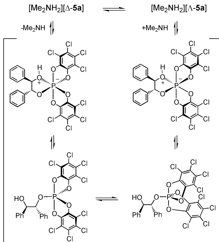
Fig. 11. Mechanistic rationale for equilibration of the diastereomers of [\text{Me}_2\text{NH}_2][\Delta\text{-5a}] salt.
