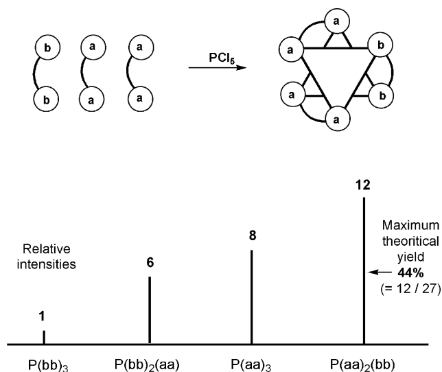
Fig. 5. Statistical distribution among possible phosphates from the reaction of two different ligands (aa and bb, 2:1 ratio) and PCl 5 .
