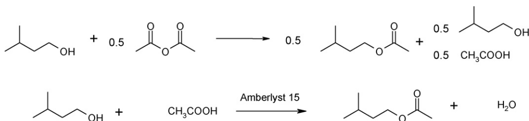
Fig. 2. Equation for esterification, with acetic anhydride as the limiting reactant.
