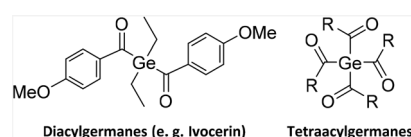
Chart 1 The state-of-the-art germanium-based photoinitiators.
