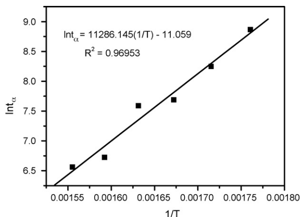
Fig. 6. Plot of \ln t_\alpha vs. 1/T for \alpha=0.4 .
