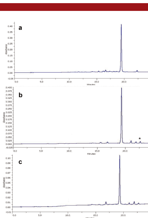
Figure 1. RP-HPLC chromatogrammes of crude reaction mixture of 5'-pT 3 obtained using (a) commercial phosphorylation reagent, (b) the present method, and (c) coinjection of both mixtures. Methylthiomethylated adduct is indicated by an asterisk (vide infra).
