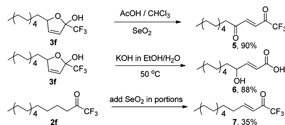
Scheme 2. Dehydrogenation of Substrate with \gamma -Hydrogen and Subsequent Conversions
