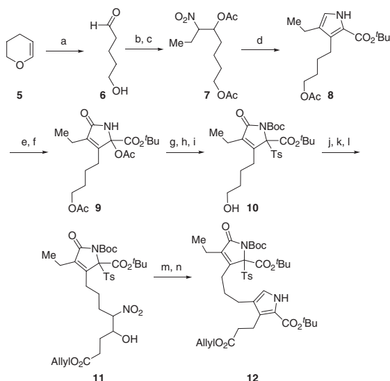
Scheme 1. a) In 0.1 M aq HCl, rt, 30 min. b) 1-Nitropropane (2.0 equiv.), KOH (0.2 equiv.) in MeOH, 0 °C–rt, 3.5 h. c) Ac 2 O (2.2 equiv.), DMAP (0.2 equiv.) in THF, 0 °C–rt, 1 h. 7 , 38% from 5 . d) CNCH 2 CO 2 - t -Bu (1.0 equiv.), DBU (2.2 equiv.) in THF, 0 °C–rt, overnight, 8 , 67%. e) NIS (1.2 equiv.) in acetone, rt, 1 h. f) Pb(OAc) 4 (1.5 equiv.) in toluene, rt, 2 d. 9 , 90% from 8 . g) TsNa (2.1 equiv.) in THF, reflux, 1.5 h. h) Boc 2 O (1.5 equiv.), DMAP (0.2 equiv.) in MeCN, –40 °C–rt, 1 h. i) In 0.5 M methanolic HCl (prepared by diluting 12 M HCl with MeOH), rt, overnight, 10 , 92% from 9 . j) I 2 (1.2 equiv.), Ph 3 P (1.2 equiv.), imidazole (2.5 equiv.) in MeCN, rt, 1 h. k) NaNO 2 (2.0 equiv.), phloroglucinol dihydrate (1.1 equiv.) in DMF, rt, 7 h. l) OHCH 2 CH 2 CO 2 -Allyl (2.0 equiv.), KOH (0.3 equiv.) in THF, 0 °C–rt, overnight, 11 , 24% from 10 . m) Ac 2 O (1.1 equiv.), DMAP (0.2 equiv.) in THF, 0 °C, 2 h. n) CNCH 2 CO 2 - t -Bu (4.0 equiv.), DBU (5.0 equiv.) in MeCN, 0 °C–rt, 4 h. 12 , 82% from 11 .
