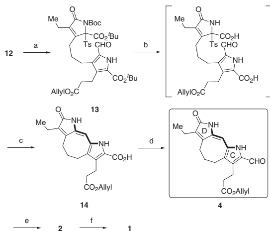
Scheme 2. a) POCl 3 (2.0 equiv.) in DMF, 65 °C, 2 h, then aq 10% NaOAc. 13 , 68%. b) 99% HCO 2 H, rt, overnight. c) n -Bu 3 P (2.5 equiv.), DBU (1.5 equiv.) in THF/DMF, –75 °C–rt, overnight. 14 , 74%. d) TFA/(MeO) 3 CH (2/1, v/v), 0 °C–rt, 1 h, then H 2 O. 4 , 40%. e) 3 , H 2 SO 4 (2.0 equiv.) in MeOH, rt, 1 h. 2 , 71%. f) [Pd(PPh 3 ) 4 ] (0.2 equiv.), TsNa (2.1 equiv.) in THF/MeOH (1/1, v/v), rt, 10 min. 1 , 70%.
