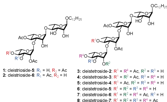
Figure 1. Targeted cleistrosides and cleistetrosides.
