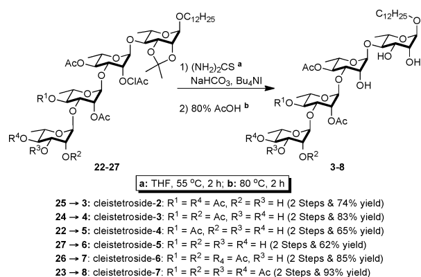
Scheme 8. Completion of the Total Synthesis of Cleistetrosides 3–8
