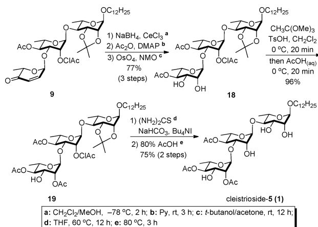
Scheme 4. Approach to Cleistrioside-5
