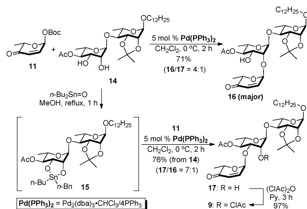
Scheme 3. Regioselective Glycosylation
