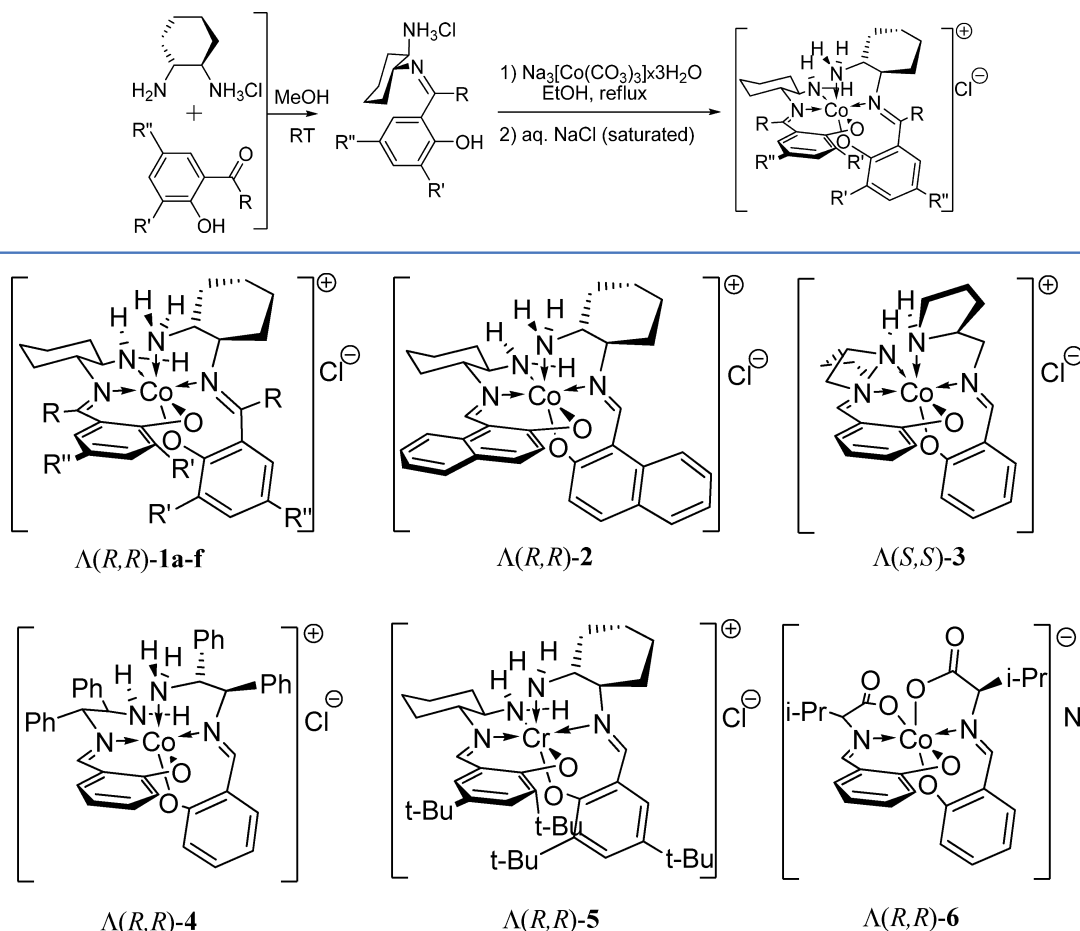
Figure 1. Structures of catalysts 1–6. (a) R = R' = R'' = \text{H} . (b) R = R'' = \text{H} , R' = \text{allyl} . (c) R = R'' = \text{H} , R' = t\text{-Bu} . (d) R = \text{H} , R' = R'' = t\text{-Bu} . (e) R' = \text{H} , R'' = \text{Ph} . (f) R = \text{Ph} , R' = R'' = \text{H} .
