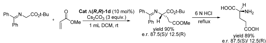
Scheme 4. Michael Addition of O'Donnell Substrate to Methyl Acrylate, Catalyzed by \Lambda(R,R) -1d
