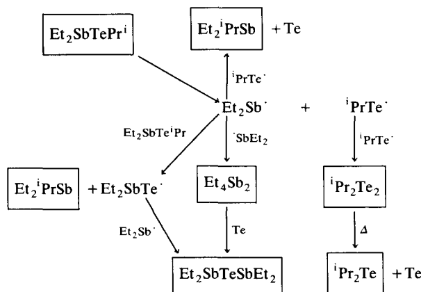
Scheme 1. Radical decomposition pathway for the compound \text{Et}_2\text{SbTe}^i\text{Pr}
