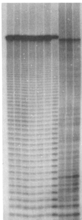
Fig. 1. Autoradiogram of crude 5'-radiolabeled oligomers obtained after deprotection of the methyl phosphate protecting groups under various conditions. 16
