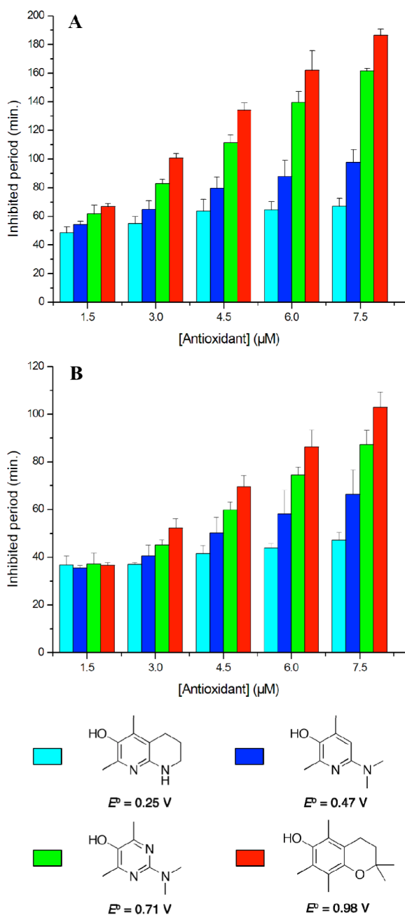
Figure 4. Inhibited periods (averages of at least three measurements) observed for pyrimidinol 1 , pyridinol 2 , naphthyridinol 12a , and PMHC as a function of antioxidant concentration when egg phosphatidylcholine liposomes were oxidized with hydrophilic (A) or lipophilic (B) peroxyl radicals. Standard potentials (vs NHE at 298 K in \text{CH}_3\text{CN} ) are given in the legend.
