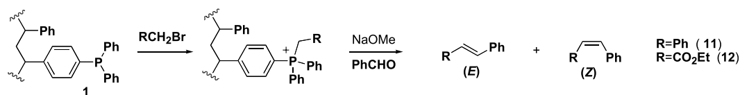
Scheme 2. Witting reaction using solid-supported triphenylphosphine ( 1b ).
