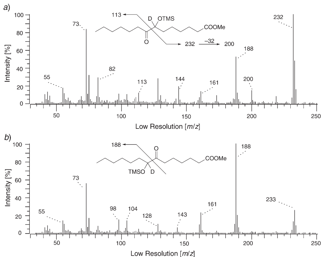
Fig. 5. Postulated EI-MS spectra of \alpha -ketols a ) 7-hydroxy-8-oxo( 7\text{-}^2\text{H}_1 )tetradecanoic acid ( 9a ) and of b ) 8-hydroxy-7-oxo( 8\text{-}^2\text{H}_1 )tetradecanoic acid ( 9b ) (methylated, silylated) isolated from cultures of S. cerevisiae after incubation of ( \pm )-erythro-7,8-dihydroxy( 7,8\text{-}^2\text{H}_2 )tetradecanoic acid ( 1 )
