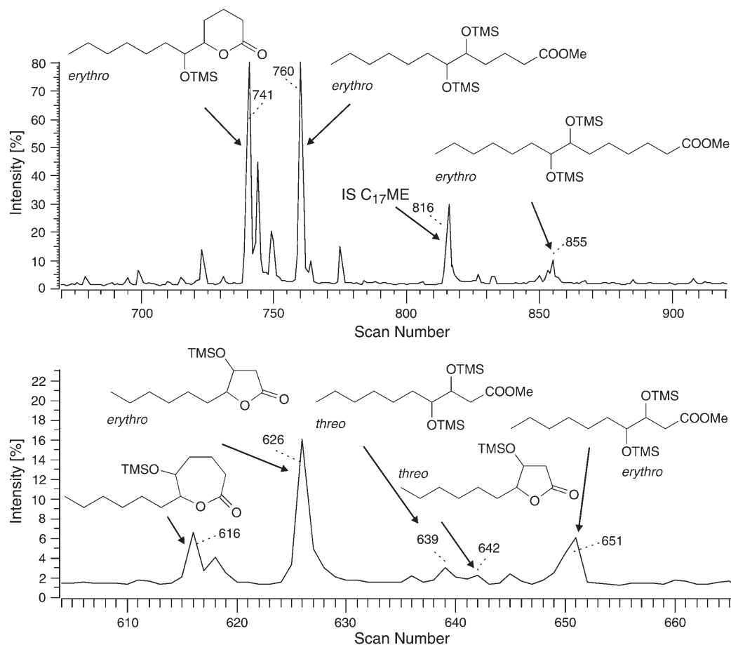
Fig. 4. GC-Chromatogram (methylated, silylated, DB-1 stationary GC phase) of metabolites isolated from the biotransformation of erythro-7,8-dihydroxytetradecanoic acid ( 1 ) (IS = internal standard: heptadecanoic acid). Traces of ( \pm )-threo-3,4-dihydroxydecanoic acid (( \pm )-threo- 2 ) and ( \pm )-threo-3-hydroxydecano-4-lactone (( \pm )-threo- 5 ) were added to emphasize the difference to the erythro-diastereoisomers.
