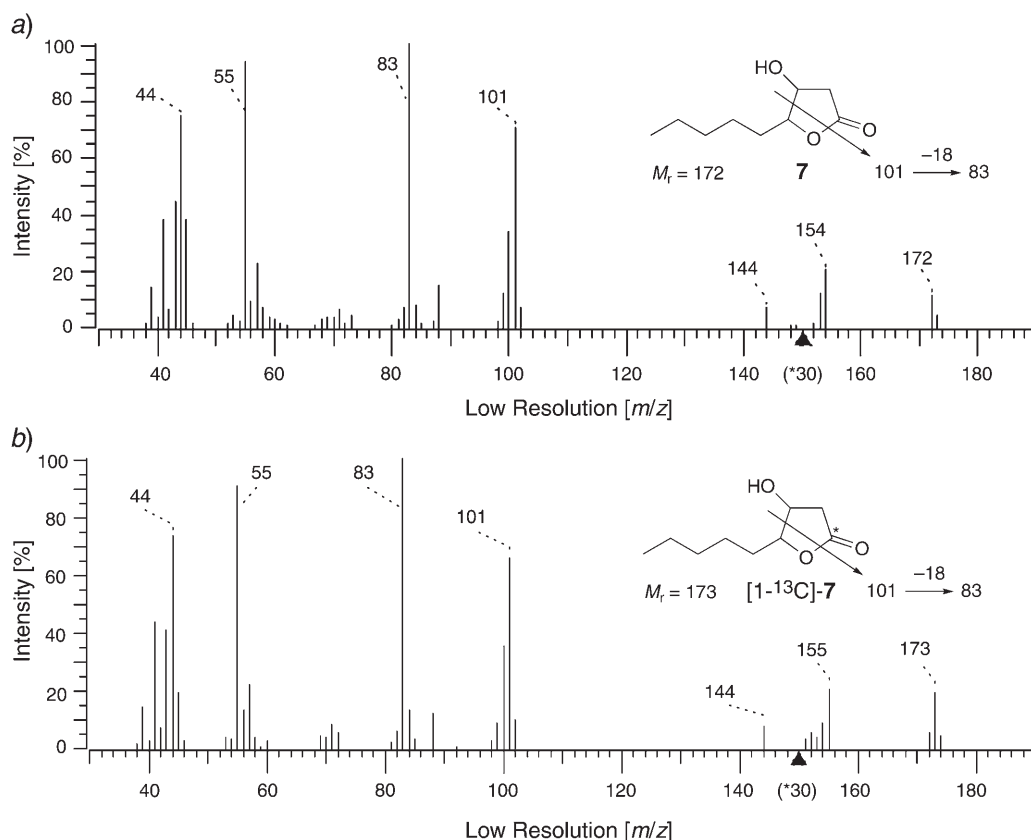
Fig. 1. EI-MS Spectra of a) unlabeled 3-hydroxynonano-4-lactone ( 7 ) and b) [1-^{13}\text{C}]\text{-7}
