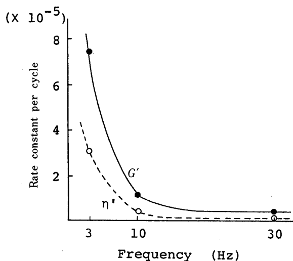
Fig. 8. Rate Constant per Cycle
