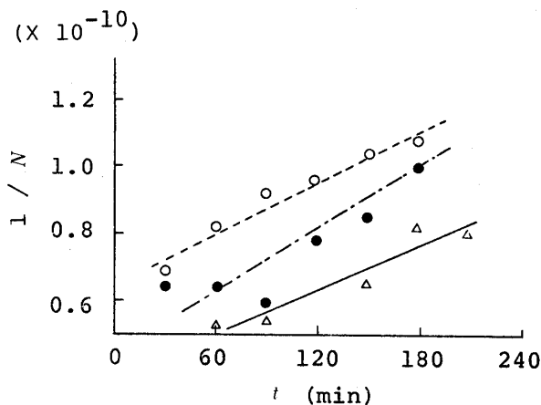
Fig. 13. Rate of Decrease in Particle Concentration as a Function of Time, Based on Eq. (1)
