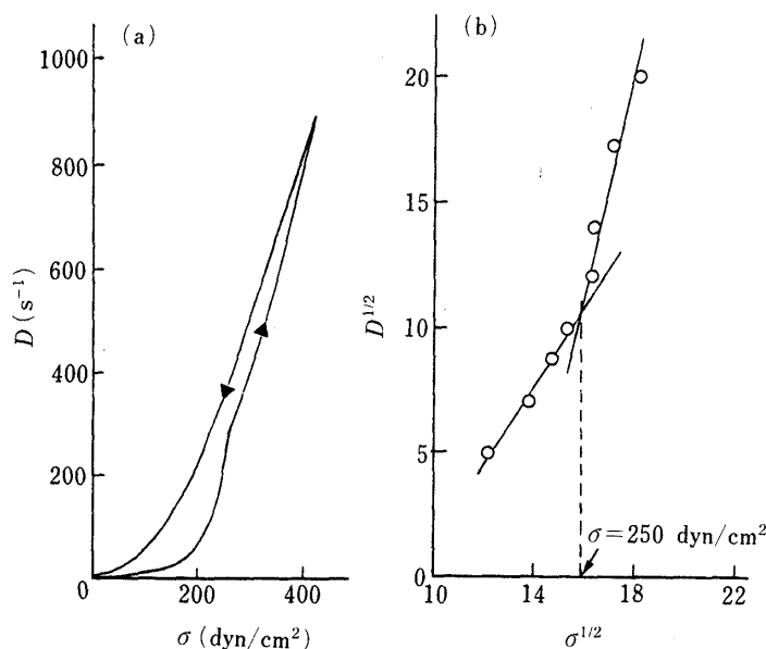
Fig. 4. (a) Flow Curve of Shear Rate, D \text{ (s}^{-1}\text{)} , versus Shear Stress, \sigma \text{ (dyn/cm}^2\text{)} , Obtained on a Cone-Plate Viscometer, and (b) Casson's Plot of D^{1/2} versus \sigma^{1/2} Obtained from the Up Curve of (a)
