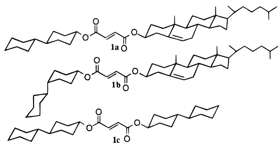
Figure 2. Fumaric acid esters primarily explored as dienophiles.
