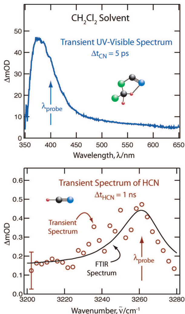
Figure 2. Top Panel: The UV-vis transient spectrum of CN radical in \text{CH}_2\text{Cl}_2 at a delay of \Delta t_{\text{CN}} = 5 ps. The structure in the panel is that of the bridging complex to which we primarily attribute this spectrum. The arrow for \lambda_{\text{probe}} marks the wavelength we use for monitoring the time evolution. Bottom Panel: The transient spectrum of HCN in \text{CH}_2\text{Cl}_2 at \Delta t_{\text{HCN}} = 1 ns. The open circles are the transient spectrum obtained from the infrared photodiode array, and the solid line is a conventional infrared spectrum obtained after a one-hour irradiation of the sample. The arrow for \lambda_{\text{probe}} marks the point we use for monitoring the time evolution, and the error bar shows the typical uncertainty for the measurements.
