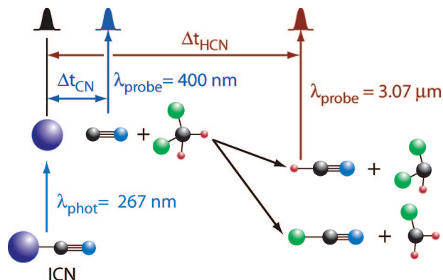
Figure 1. Experimental approach for transient absorption studies of CN reactions. A \lambda_{\text{phot}} = 267 \text{ nm} photolysis pulse dissociates the ICN precursor, and probe pulses at either \lambda_{\text{probe}} = 400 \text{ nm} or \lambda_{\text{probe}} = 3.07 \mu\text{m} interrogate the CN reactant or the HCN product respectively, at time delays of \Delta t_{\text{CN}} or \Delta t_{\text{HCN}} following the photolysis pulse. Hydrogen abstraction from \text{CH}_2\text{Cl}_2 is exothermic by 9700 \text{ cm}^{-1} , and chlorine abstraction from \text{CH}_2\text{Cl}_2 is exothermic by 6000 \text{ cm}^{-1} .
