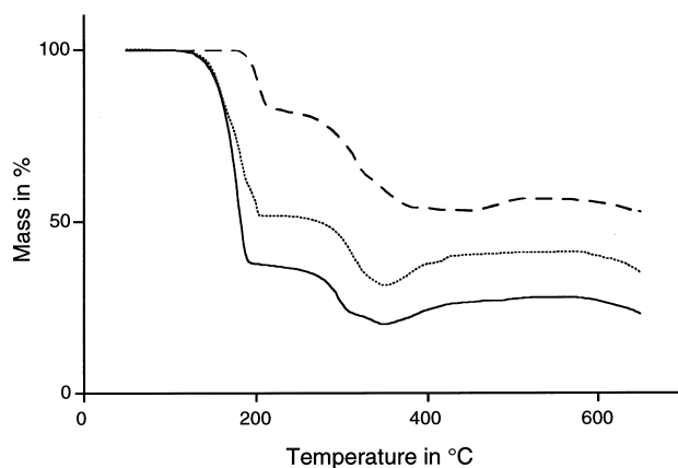
Fig. 5. The TG curves of \text{Cu}_2(\text{DMDTO})\text{Cl}_2 (---), \text{Cu}(\text{DMDTO})\text{Cl} (···) and \text{Cu}(\text{DMDTO})_2\text{Cl} (—).
