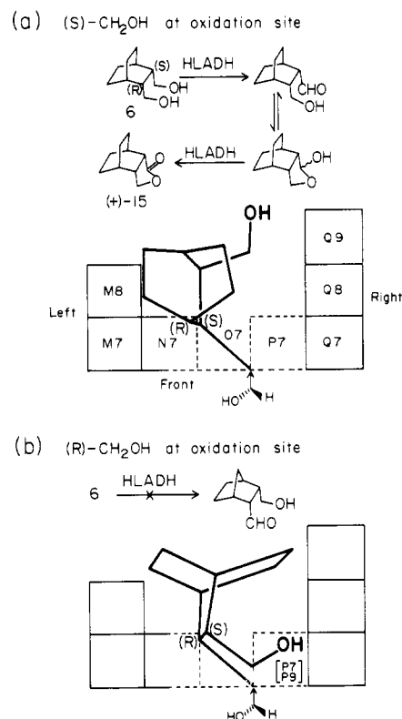
Figure 1. Cubic active-site section analysis of the stereospecificity of HLADH-catalyzed oxidation of the [2.2.2] diol 6. The model, the alpha-numeric descriptors of the cube locations, and the analytical procedure employed are as described previously. 13 The substrate orientations in this analysis are depicted from the top elevation 13 perspective. Cubes bounded by solid lines are "forbidden" regions where the presence of the coenzyme or amino acid residues of the enzyme preclude accommodation of the substrate. The space above, underneath, and in front of the defined active-site region are forbidden for the same reasons. Substrate binding in cubes bordered by broken lines is "limited" by the proximity of these spaces to forbidden regions. Substrates can locate in limited space but the binding is not favored. Violation of two limited regions becomes equivalent to a forbidden interaction. The open areas are "allowed" regions where the substrate can be freely accommodated. For oxidation to occur, the hydroxyl group must locate at the oxidation site, identified by \rightarrow . For primary alcohols, HLADH-catalyzed oxidation requires abstraction of the pro-R hydrogen atom, 13,14 thereby ensuring a unique CH 2 OH orientation. The substrate orientations shown are the most favorable in (a) and the least unfavorable in (b). In (a), for oxidation of the CH 2 OH group attached to the S center, all of the substrate can locate in allowed regions and oxidation proceeds readily. In (b), no orientations are possible that do not involve unfavorable interactions. In the least unfavorable fit shown, the penetration of limited regions P7 and P9 cannot be avoided. Furthermore, these regions are hydrophobic and the location of a polar hydroxyl group here would be particularly unpropitious. Productive ES complex formation is therefore precluded and oxidation does not occur.
