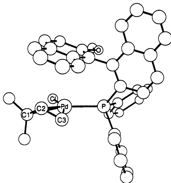
Figure 1. Molecular structure of 4a . Selected bond distances (Å) and angles (deg): Pd–C1, 2.304(4); Pd–C2, 2.152(5); Pd–C3, 2.110(6); Pd–Cl, 2.387(1); Pd–P, 2.3098(9); C1–C2–C3, 122.6(4); C1–Pd–C2, 36.5(2); C2–Pd–C3, 38.7(2); C1–Pd–C3, 67.9(2); C1–Pd–Cl, 90.3(2); Cl–Pd–P, 105.26(4); C3–Pd–P, 95.5(1). Twist angle between two naphthyls, 85.2(8)^\circ .
