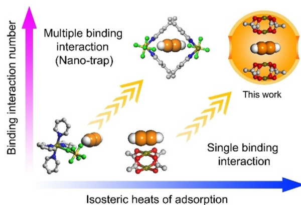
Scheme 1. The multiple interactions strategy for enhancing binding interaction between C_2H_2 and binding site.
