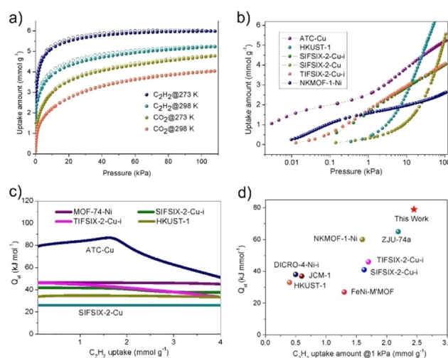
Figure 2. a) The C 2 H 2 and CO 2 isotherms for ATC-Cu at 273 K and 298 K. b) The C 2 H 2 adsorption isotherms for ATC-Cu and high performance MOFs at 298 K. c) The Q_{st} for ATC-Cu and high performed MOFs. d) The Q_{st} against C 2 H 2 uptake amount at 1 \times 10^{-2} bar for high-performance acetylene adsorbent.
