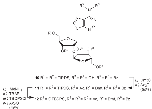
Scheme 3. Introduction of Orthogonal Protective Groups
