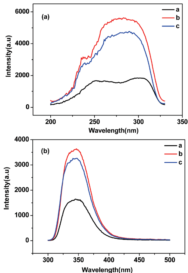
Figure 12. Excitation (a) and emission (b) spectra of the products with different morphologies: a, flower-like hierarchical architectures (S3, Figure 3c); b, prisms (3.8 mL \text{HNO}_3 , Figure 6d); c, nanorods (0 g citric acid, Figure 7a). (The three samples are measured by using the same experimental conditions.)
