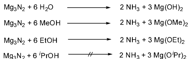
Figure 1. Reaction of \text{Mg}_3\text{N}_2 with various proton sources.
