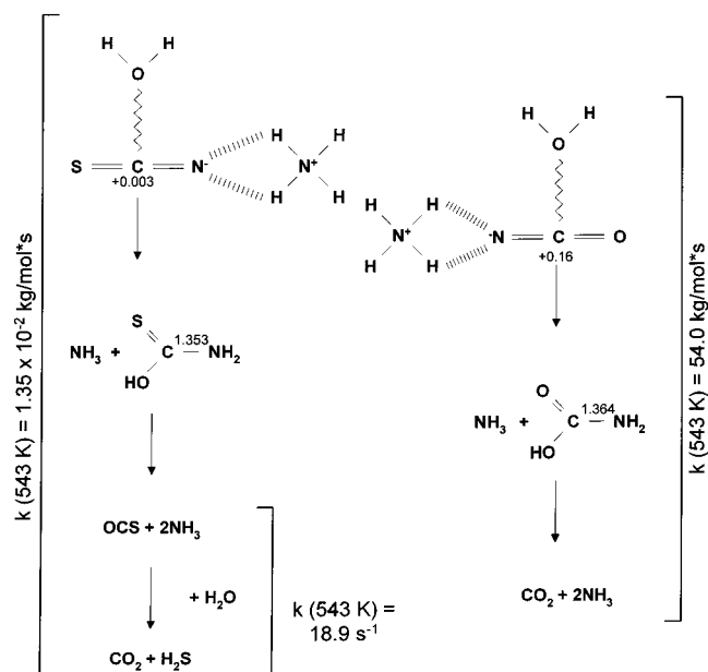
Figure 5. Proposed hydrothermolysis pathway for aqueous \text{NH}_4\text{SCN} and \text{NH}_4\text{OCN} showing charges and bond parameters (Å) from ab initio quantum mechanical calculations and rate comparisons at 543 K under 275 bar.
