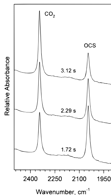
Figure 4. Mid-IR spectra of approximately 0.25 M \text{OCS} during hydrothermolysis at 493 K and 275 bar at several residence times in the 316 SS flow reactor.
