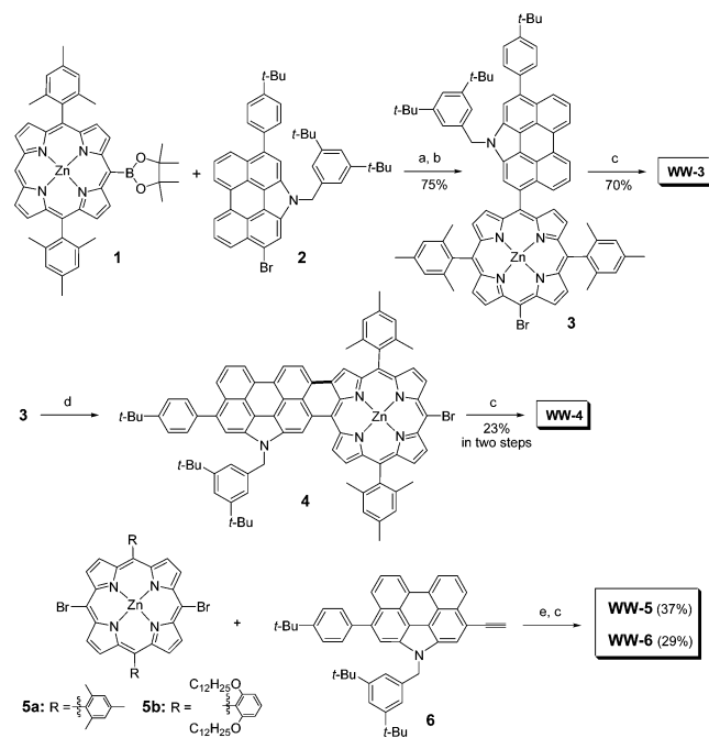
Scheme 1. Synthesis of N -Annulated Perylene-Substituted and Fused Porphyrin Dyes WW-3–WW-6: (a) Pd(PPh 3 ) 4 , Cs 2 CO 3 ; (b) NBS, CHCl 3 ; (c) 4-ethynylbenzoic acid, Pd(PPh 3 ) 4 , CuI, TEA; (d) FeBr 3 , 1,2-dichloroethane; (e) Pd(PPh 3 ) 4 , CuI, TEA
