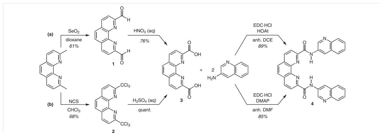
Scheme 1 (a) The first three steps in the previously reported synthesis of bisquinolinium ligand Phen-DC3 (41% overall yield). 7 (b) Synthesis of compound 4 via chlorinated intermediate compound 2 , with an overall yield of 58%.
