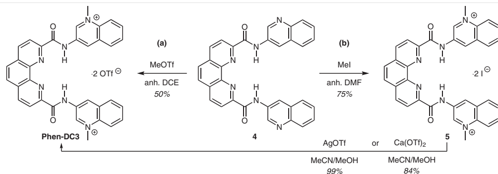
Scheme 2 Synthesis of Phen-DC3 via (a) the reported methylation of compound 4 using methyl triflate, 7 and (b) the proposed alternate strategy involving the use of methyl iodide as methylating agent, which affords the diiodide salt in good yield, followed by metathesis in cases where exchange of counterions is necessary.
