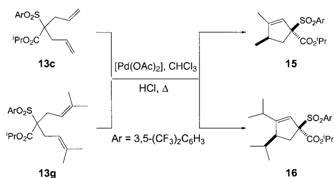
Scheme 4. Cycloisomerization Reactions
