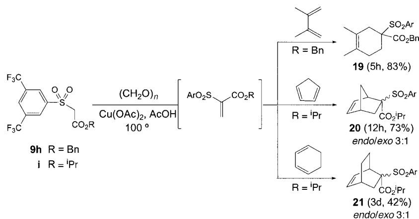
Scheme 6. Diels-Alder Cycloadditions
