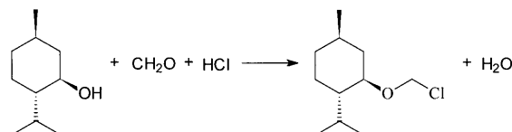
Scheme 4. Chloromethylation of (1 R ,2 S ,5 R )-(–)-menthol.
