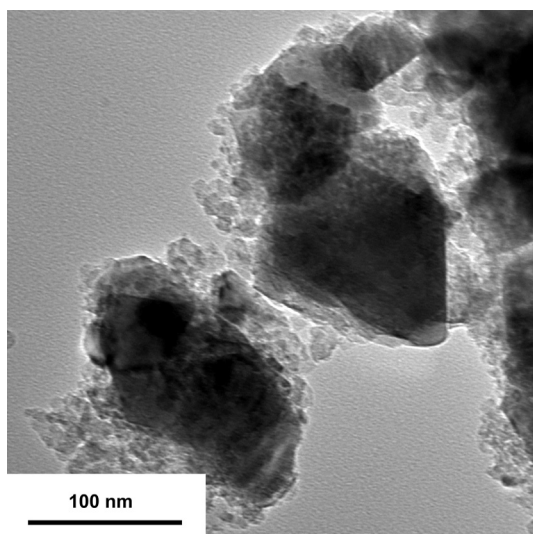
Fig. 5. TEM image of the T3(17) catalyst.
