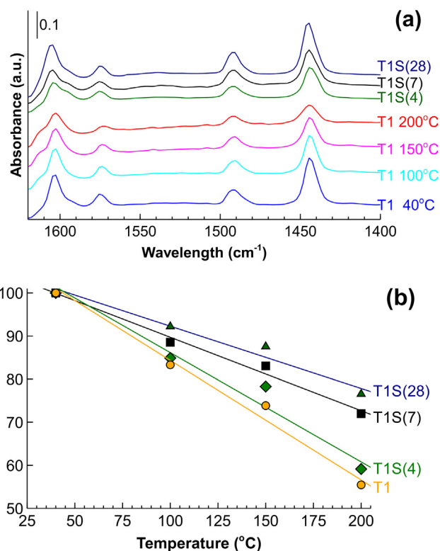
Fig. 13. (a) FTIR spectra of pyridine over sulfated titania catalysts and (b) temperature dependence of the normalized intensity of the 1445\text{ cm}^{-1} band at 40^\circ\text{C} .
