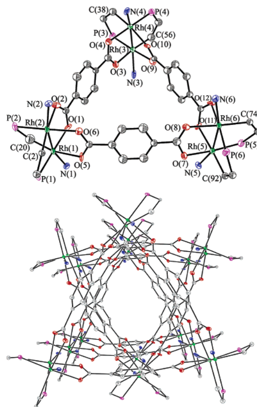
Figure 2. The core structure (top) and packing pattern (bottom) of SSS-3 . Displacement ellipsoids for the core structure are drawn at the 40% probability level. Some carbon atoms in phosphine groups and pyridine ligands, solvent molecules, and hydrogen atoms are omitted for clarity. Note that molecules stack on top of each other, but out of register, leaving a chiral channel.
