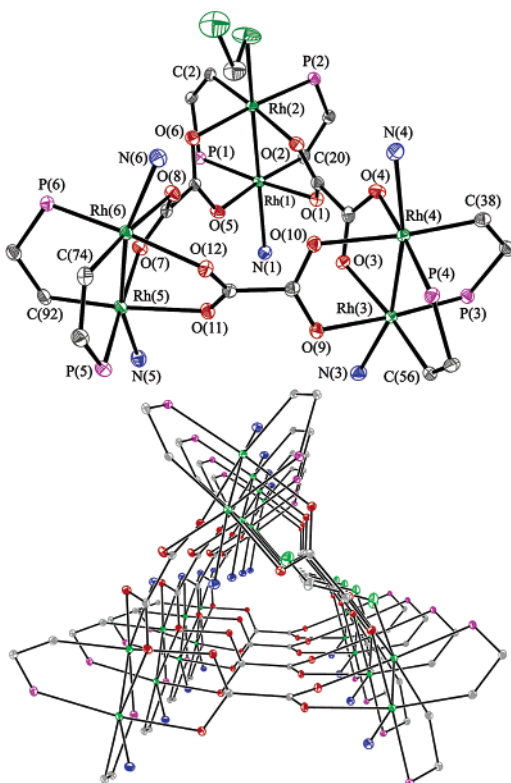
Figure 3. The core structure (top) and packing pattern (bottom) of SSS-4. Displacement ellipsoids for the core structure are drawn at the 40% probability level. Some carbon atoms in phosphine groups and pyridine ligands, solvent molecules, and hydrogen atoms are omitted for clarity. Note that all molecules stack, leaving a chiral channel.
