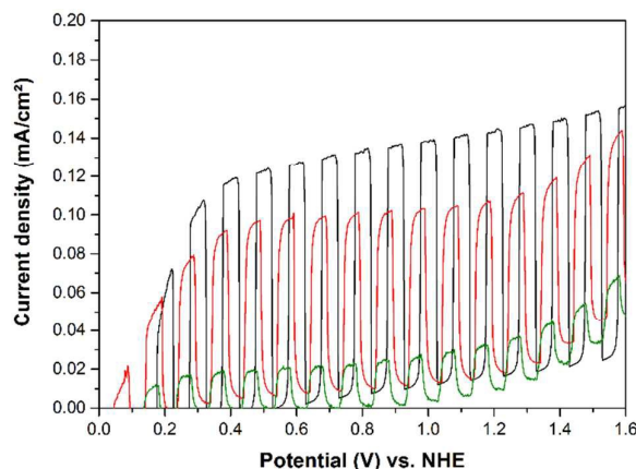
Figure 5. Chopped light current-potential curves of cold sprayed \text{TiO}_2 on titanium metal (red), screen printed \text{TiO}_2 on FTO (black) and screen printed \text{TiO}_2 on titanium metal (green) photoanodes in 0.5 M \text{H}_2\text{SO}_4 with a scan rate of 20 mV/s. Current densities were measured upon irradiation with AM 1.5-global light (300 W Xe lamp).
