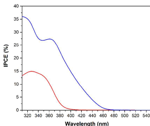
Figure 13. IPCE spectra for water oxidation employing cold sprayed \text{WO}_3 (blue) and \text{TiO}_2 (red) on titanium metal photoanodes. Measurements for water oxidation were conducted in an aqueous 0.5 M \text{H}_2\text{SO}_4 solution at a bias of 1 V vs. NHE.
