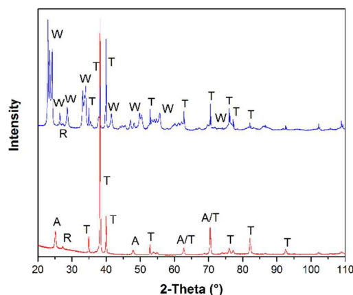
Figure 2. XRD patterns of \text{WO}_3 (blue) and \text{TiO}_2 (red) films deposited on titanium metal substrates by cold spray, where W denotes for \text{WO}_3 pattern, T for titanium metal pattern, R for rutile \text{TiO}_2 pattern and A for anatase \text{TiO}_2 pattern.
