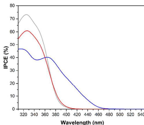
Figure 14. IPCE spectra for methanol oxidation employing cold sprayed \text{WO}_3 (blue) and \text{TiO}_2 (red) on titanium metal photoanodes. The IPCE curve of screen printed \text{TiO}_2 on FTO photoelectrode is also given (light grey) for comparison. Measurements for methanol oxidation were conducted in an aqueous solution of 0.5 M \text{H}_2\text{SO}_4 with addition of 10 vol-% of methanol ( \sim 2 mol/L) at a bias of 1 V vs. NHE.
