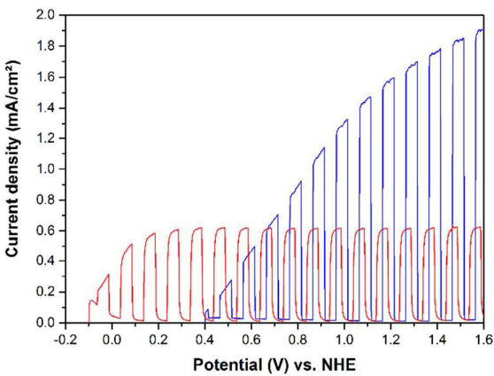
Figure 12. Chopped light current-potential curves of cold sprayed WO 3 (blue) and TiO 2 (red) on titanium metal photoanodes in 0.5 M H 2 SO 4 with addition of 10 vol-% of methanol (~ 2 mol/L). Measured with a scan rate of 20 mV/s. Current densities were measured upon irradiation with AM 1.5-global light (300 W Xe lamp).
