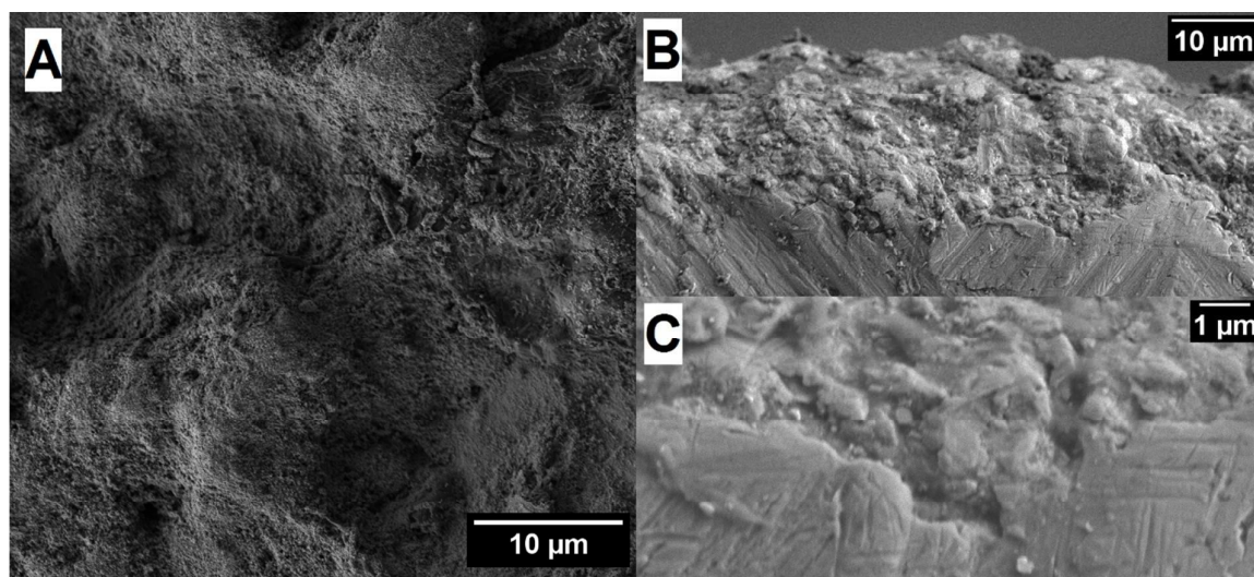
Figure 4. A) SEM surface morphology image of a cold sprayed TiO 2 film. B) Cross-sectional SEM image of a cold sprayed WO 3 film on a titanium substrate at a magnification of 1400x. C) Cross-
