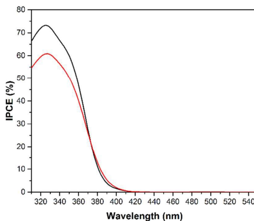
Figure 8. IPCE spectra for methanol oxidation measured for cold sprayed P25/20 on titanium metal (red) and screen printed P25 on FTO (black) photoanodes. Measurements for methanol oxidation were conducted in an aqueous solution of 0.5 M H 2 SO 4 with addition of 10 vol-% of methanol (~ 2 mol/L) at a bias of 1 V vs. NHE.
