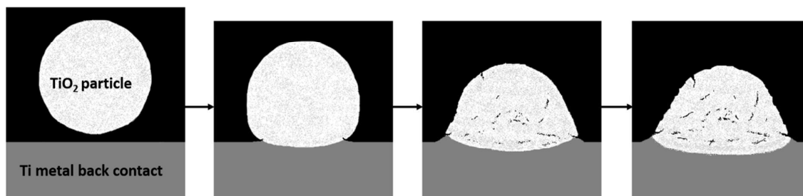
Figure 1. Scheme of the impact of a \text{TiO}_2 cold sprayed particle (white) on a Ti metal substrate (grey). The powder particle deforms and partially cracks during impact while the metal substrate deforms plastically. As a result, the \text{TiO}_2 particle is bonded to the metal without the help of any additive or binder.
