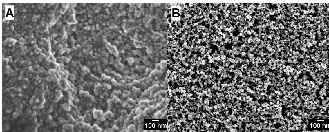
Figure 5. A) SEM image of a cold sprayed \text{TiO}_2 (P25/20) film on Ti metal substrate. B) SEM image of a screen printed \text{TiO}_2 (P25) film on FTO substrate.
