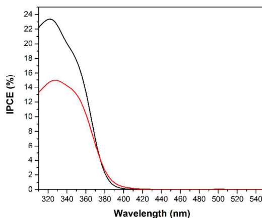
Figure 7. IPCE spectra for water oxidation measured for cold sprayed TiO 2 on titanium metal (red) and screen printed TiO 2 on FTO (black) photoanodes. Measurements for water oxidation were conducted in an aqueous 0.5 M H 2 SO 4 solution at a bias of 1 V vs. NHE.
