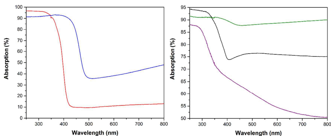
Figure 3. Absorption spectra of the employed WO 3 (blue) and TiO 2 P25/20 (red) powders (left side) and of the cold sprayed Ti/WO 3 (green) and Ti/TiO 2 (black) photoelectrodes (right side). The purple curve on the right side shows the absorption spectra of the employed blank Ti substrate.
