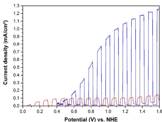
Figure 9. Chopped light current-potential curves of cold sprayed \text{WO}_3 (blue) and \text{TiO}_2 (red) on titanium metal photoanodes in 0.5 M \text{H}_2\text{SO}_4 with a scan rate of 20 mV/s. Current densities were measured upon irradiation with AM 1.5-global light (300 W Xe lamp).
