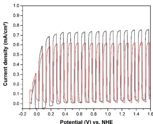
Figure 6. Chopped light current-potential curves of cold sprayed TiO 2 on titanium metal (red) and screen printed TiO 2 on FTO (black) photoanodes in 0.5 M H 2 SO 4 with addition of 10 vol-% of methanol (~2 mol/L). Measured with a scan rate of 20 mV/s. Current densities were measured upon irradiation with AM 1.5-global light (300 W Xe lamp).
