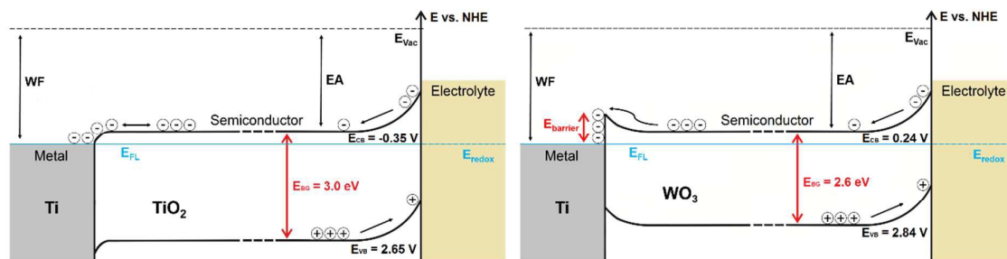
Figure 15. Schematic energy band diagram for n-type semiconductor photoelectrodes under illumination and after the equilibration of Fermi levels at the metal-semiconductor and the semiconductor-electrolyte interfaces with the appearance of band bending. For the Ti/WO 3 junction a Schottky contact is assumed, while for the Ti/TiO 2 junction an Ohmic contact is readily expected. The theoretical Schottky barrier height for the Ti/WO 3 junction is \Delta\Phi \approx 0.8 eV.
