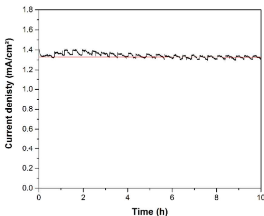
Figure 11. Polarization curve of cold sprayed \text{WO}_3 on titanium metal photoanode in 0.5 M \text{H}_2\text{SO}_4 with addition of 10 vol-% of methanol ( \sim 2 mol/L). Measured at a constant anodic potential of 1 Volt vs. NHE over 10 hours. Current densities were measured upon irradiation with AM 1.5-global light (300 W Xe lamp). A linear fit (red) was made after 6 hours to estimate the stability of the photocurrent. The slope of the fitting curve is -4.137 \times 10^{-4}\ \text{mA}/\text{h} \cdot \text{cm}^2 .
