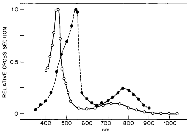
Figure 3. The photodissociation cross section of the molecular cation (○) from cis -stilbene and the matrix absorption spectrum of cis -stilbene radical cation (●).
