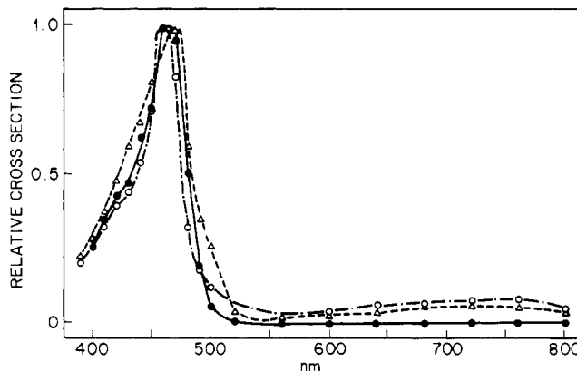
Figure 2. The photoformation cross sections of 2 (○), 3 (●), and 4 (Δ). The spectra are normalized relative to their maxima for comparison.
