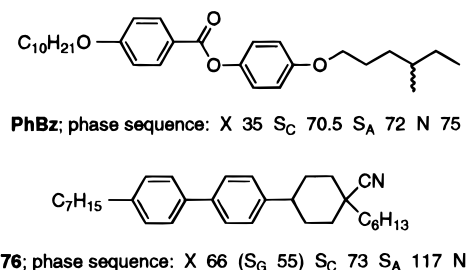
Figure 2. Structures of S_C hosts and phase transition temperatures in °C.
