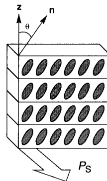
Figure 1. Schematic representation of the SSFLC. The polar axis is \perp to the plane of the page.
