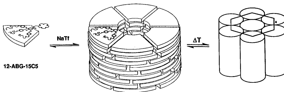
Scheme 2. Synthesis of 12Fn-AG-15C5 (4-m/n) and 12F8-AG-B15C5 (5-4/8)
