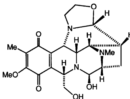
3, NAPHTHYRIDINOMYCIN
