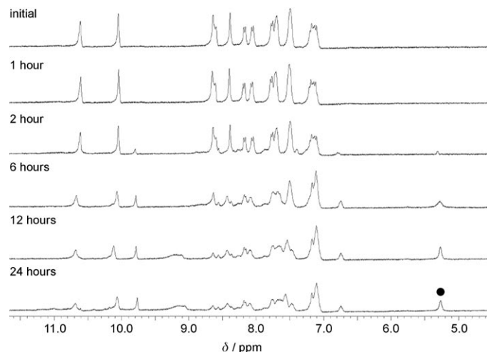
Figure 6. Decomposition of a solution of receptor 2 (1.0 mM) in [\text{D}_6]\text{DMSO}/0.5\% water at 25^\circ\text{C} as shown by ^1\text{H} NMR spectroscopy. The marked resonance corresponds to free \text{NH}_2 shown in structure of 9 .
