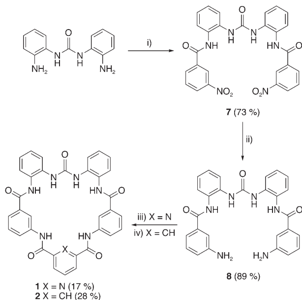
Scheme 1. The synthesis of macrocycles 1 and 2 . i) 3-nitrobenzoic acid, PyBOP, \text{Et}_3\text{N} , HOBt, DMF (anhydrous); ii) \text{NH}_2\text{NH}_2\cdot\text{H}_2\text{O} , Pd/C 10% cat., EtOH; iii) 2,6-pyridine dicarbonylchloride, tetrabutylammonium acetate, \text{Et}_3\text{N} , DMAP, \text{CH}_2\text{Cl}_2 ; iv) isophthaloyl dichloride, \text{H}_2\text{SO}_4 , MeOH.
