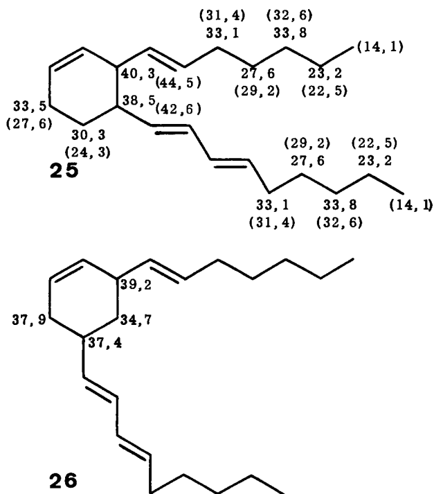
Fig. 4. Calculated ^{13}\text{C} chemical shift values for 25 and 26 . In brackets: experimental values favoring 25
