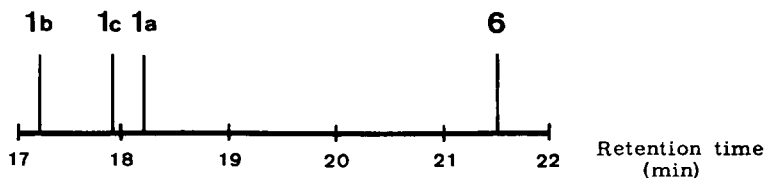
Fig. 1. Gas chromatography of the trienes 1a–c and 6 using an Apiezon glass capillary column (0.31 mm \times 50 m) at 120^\circ (He pressure 0.55 atm) on a Carlo Erba GI apparatus
