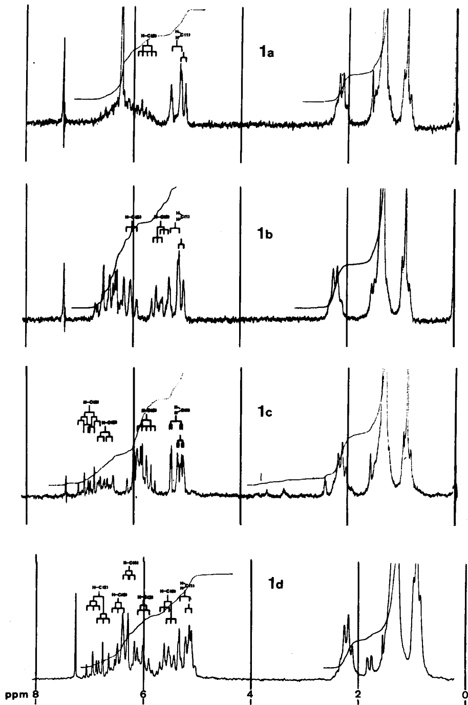
Fig. 2. 90\text{ MHz } ^1\text{H-NMR} spectra (in \text{CDCl}_3 ) of 1a-d
