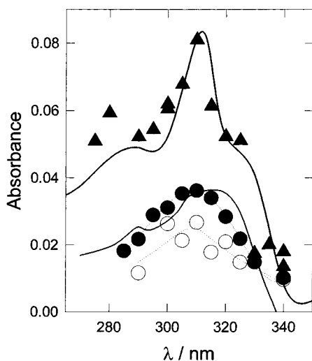
Figure 5. Absorption spectrum of the organic transients obtained 250 \mu\text{s} after irradiation with a conventional flash lamp for \text{N}_2 ( \blacktriangle ), air ( \bullet ) and \text{O}_2 ( \circ )-saturated 5 mM \text{K}_2\text{S}_2\text{O}_8 solutions containing 0.5 M NaCl in the presence of 5.6 mM toluene. The solid line corresponds to the normalized published spectrum of the HO-CHD radicals of toluene from refs 27 (upper spectrum) and 26, 28] (lower spectrum).
