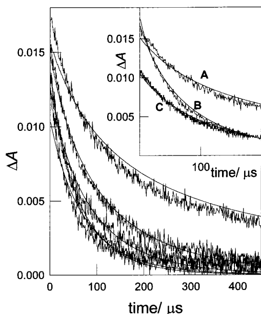
Figure 1. Signals obtained at \lambda_{\text{obs}} = 340 nm by laser flash photolysis experiments with 25 mM \text{K}_2\text{S}_2\text{O}_8 and 49.2 mM \text{NaCl} solutions containing variable concentrations of chlorobenzene from up to down: 0, 1.3, 2.17, 2.82, and 3.47 mM. Inset: Idem for solutions containing 25 mM \text{K}_2\text{S}_2\text{O}_8 and (a) [\text{ClBz}] = 0 M, [\text{Cl}^-] = 0.069 M; (b) [\text{ClBz}] = 2.8 mM, [\text{Cl}^-] = 69 mM; and (c) [\text{ClBz}] = 2.8 mM, [\text{Cl}^-] = 96.2 mM. The solid lines represent computer simulations (refer to text).
