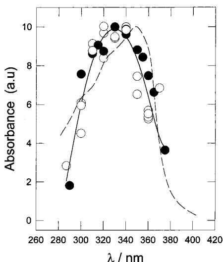
Figure 4. Absorption spectrum of the organic transients obtained 200 \mu s after irradiation with a conventional flash lamp, of nitrogen-saturated solutions containing 5 mM \text{K}_2\text{S}_2\text{O}_8 and 0.05 M (O) or 0.1 M (●) NaCl in the presence of 7.2 mM benzoic acid. The dashed line corresponds to the normalized reported spectrum of the HO-CHD radicals of benzoic acid. 16
