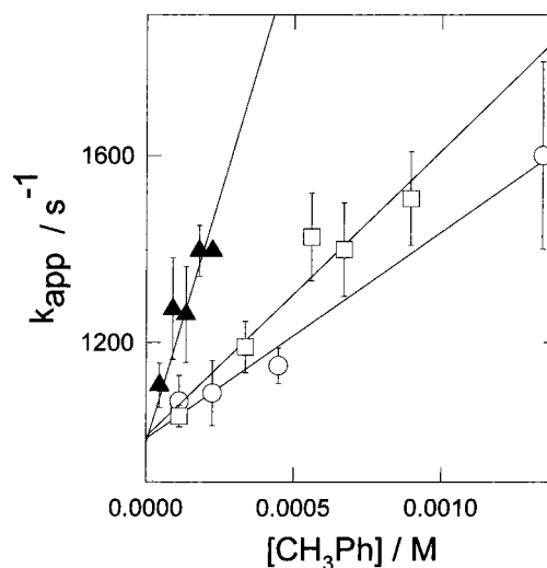
Figure 2. Linear dependence of the first-order decay component ( k_{\text{app}} ) of \text{Cl}_2^{\bullet-} on [\text{CH}_3\text{Ph}] for experiments with [\text{Cl}^-] = 0.1 M (▲), 0.2 M (□), and 0.4 M (○).
