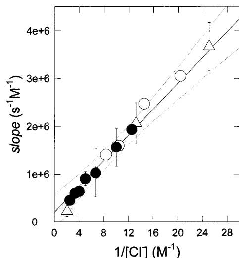
Figure 3. Dependence of the slopes of the plots of k_{\text{app}} vs [\text{XPh}] on [\text{Cl}^-]^{-1} for (●) toluene, (Δ) benzoic acid, and (○) chlorobenzene. Since the organic radical ( \text{R}^{\bullet} ) formed from benzoic acid shows significant absorption at 340 nm (vide infra), the observation wavelength for the experiments done with this substrate was 360 nm.
