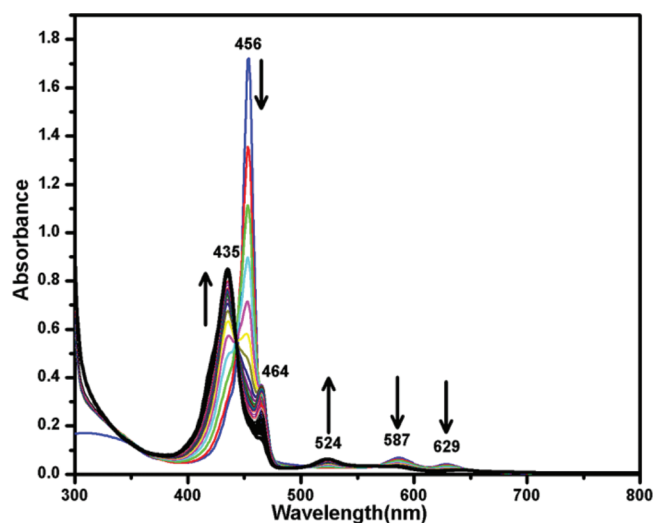
Figure 6. Electronic spectral changes in 16 h of 2 (blue) after the addition of excess benzenethiol in toluene. The band at 464 nm is indicative of the intermediate species [W^V O(TPP)(SPh)] .
