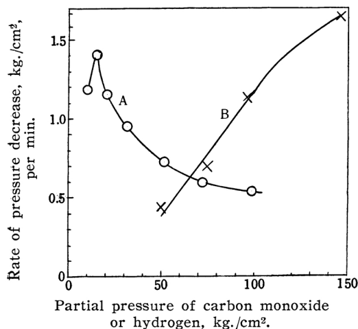
Fig. 2. Relation of rate of hydroformylation to partial pressure of carbon monoxide (A) or hydrogen (B). A: hydrogen partial pressure, 97 kg./cm². B: carbon monoxide partial pressure, 21 kg./cm².
