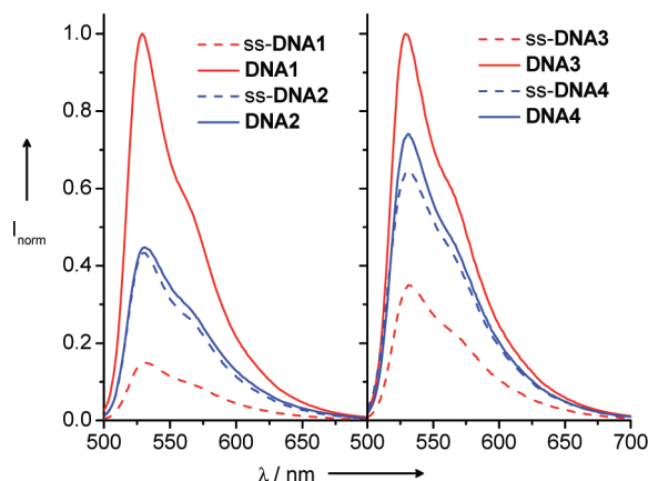
FIGURE 1. Fluorescence spectra of DNA1–DNA4 (2.5 \mu M), 10 mM Na-P i -buffer (pH 7.0), 250 mM NaCl, 20 °C, \lambda_{\text{exc}} = 490 nm.
