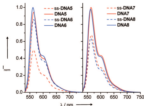
FIGURE 2. Fluorescence spectra of DNA5–DNA8 (2.5 \mu M), 10 mM Na-P i -buffer (pH 7.0), 250 mM NaCl, 20 °C, \lambda_{\text{exc}} = 530 nm.
