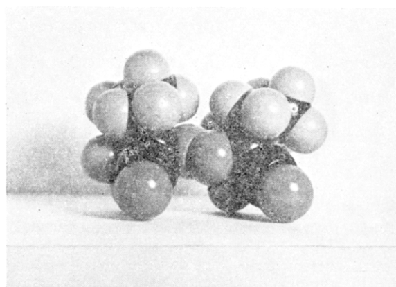
Fig. 4.—1,1'-Azo-1-cyclohexane nitrile.
