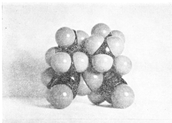
Fig. 3.—2,2'-Azo-bis-2,4-dimethylvaleronitrile ( meso form).
