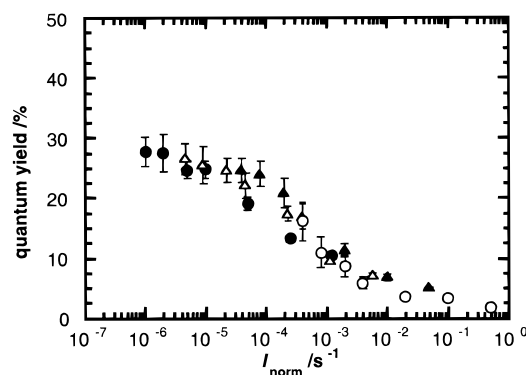
Figure 6. Plots of QY values vs log I_{\text{norm}} (s -1 ), a parameter that is defined as the ratio of the number of absorbed photons to the number of adsorbed 2-propanol molecules (initial 2-propanol concentration: ● 1000 ppmv, △ 100 ppmv, ▲ 10 ppmv, ○ 1 ppmv).
