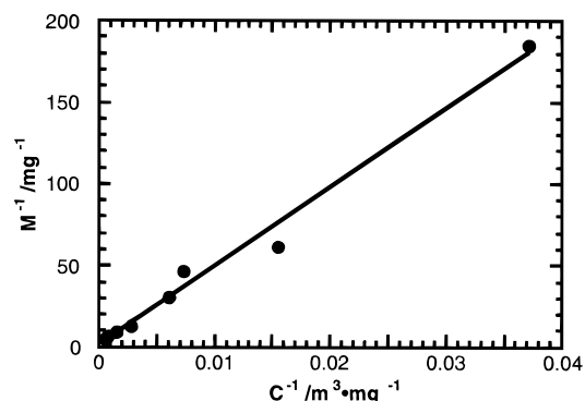
Figure 1. Inverse plots of the gaseous concentration ( C/\text{mg}\cdot\text{m}^{-3} ) and the weight of adsorbed 2-propanol ( M/\text{mg} ) on the \text{TiO}_2 thin film used for analysis of the Langmuir-type isotherm.
