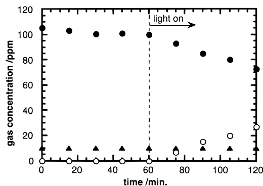
Figure 2. Concentration changes of gaseous 2-propanol, acetone, and \text{CO}_2 as a function of time in the decomposition of gaseous 2-propanol (incident UV intensity, 45 \mu\text{W}\cdot\text{cm}^{-2} ; initial 2-propanol concentration, 100 ppmv; ● 2-propanol, ○ acetone, ▲ carbon dioxide).
