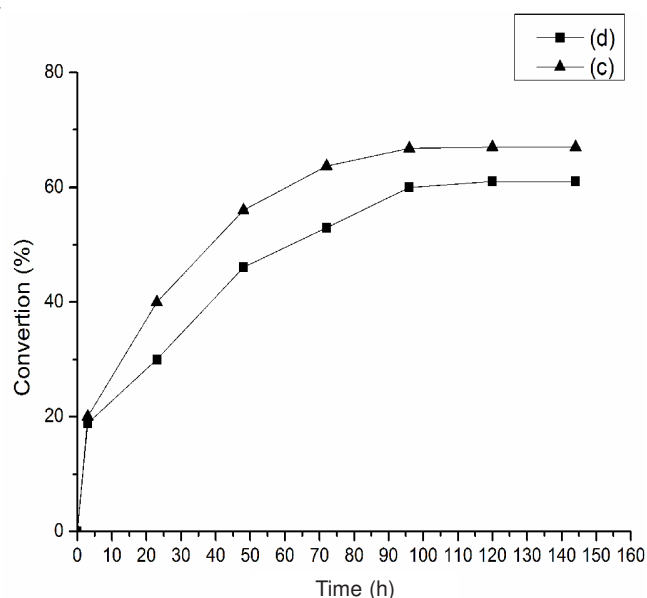
Fig. 5. Conversion yield of Novozyme 435 catalyzed by (3) and (4) at the pH = 6.5 and the temperature 30 °C
