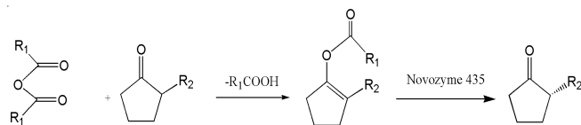
Fig. 1. Synthesis of enol ester and preparation of (R)-2-alkylcyclopentanone
